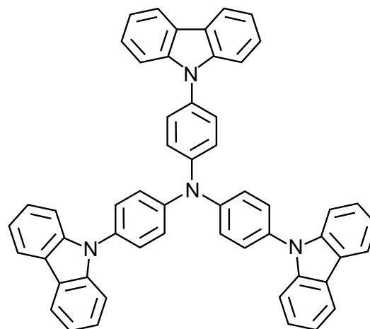
4,4',4''-tri-9-carbazolyltriphenylamine
