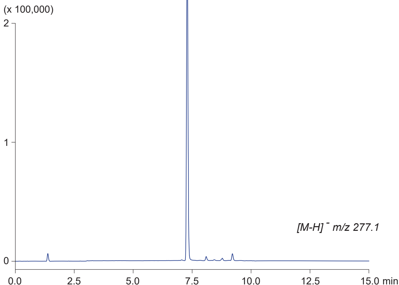
5-propyl-3,8-dimethyl- 1-azulenesulfonic acid (gualenic acid)
