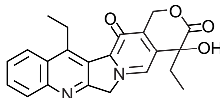
7-ethylcamptothecin
