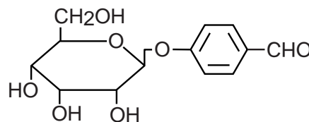
4-formylphenyl beta-D-allopyranoside (helicide)
