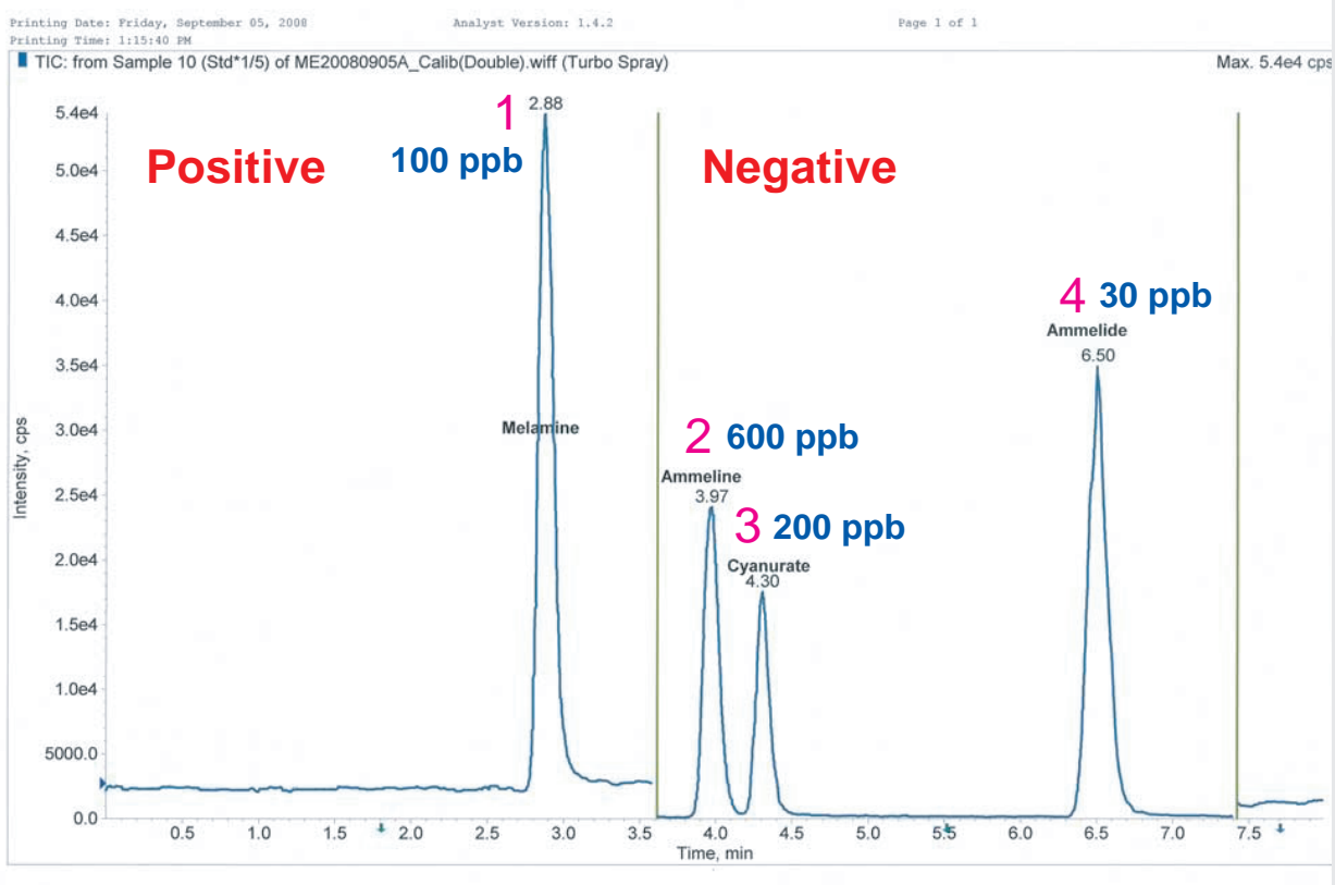
3. cyanuric acid
