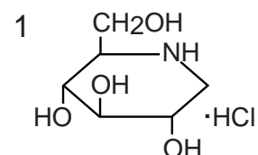
1-deoxynojirimycin hydrochloride
