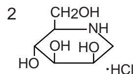
1-deoxymannojirimycin hydrochloride
