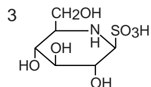
nojirimycin bisulfite
