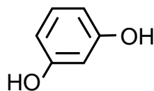
resorcinol
