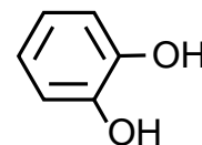
catechol (pyrocatechol)
