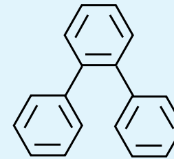
1 o -terphenyl
