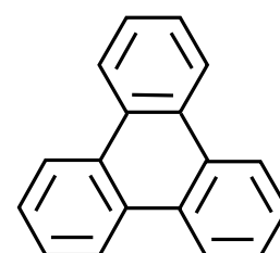
2 triphenylene
