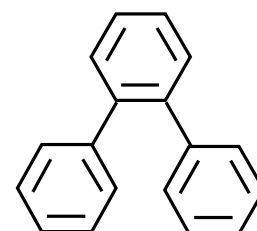
1 o -terphenyl
