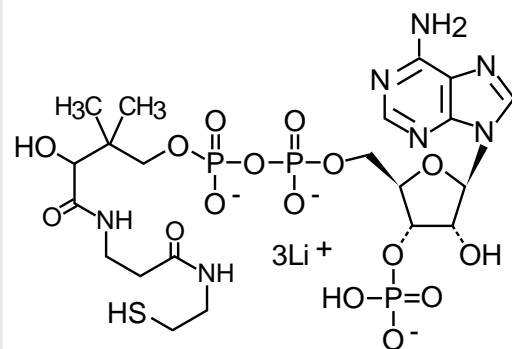
1 coenzyme A (CoA)
