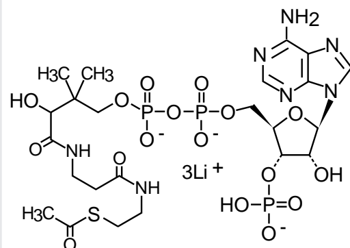
2 acetyl coenzyme A (Acetyl-CoA)
