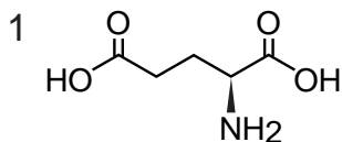
L-glutamic acid
