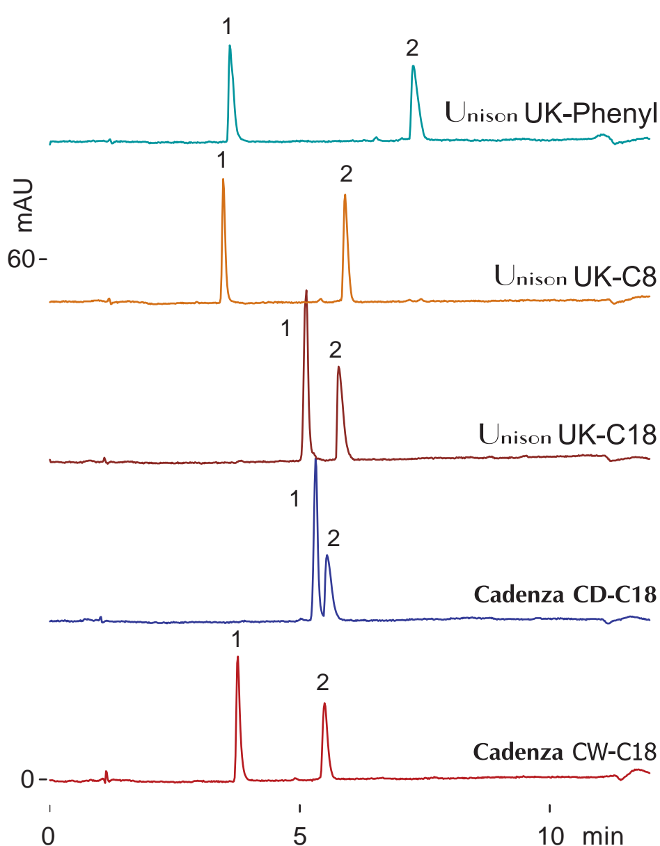
leucomalachite green
