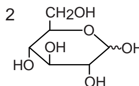
D-glucose
