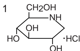
1-deoxynojirimycin hydrochloride
